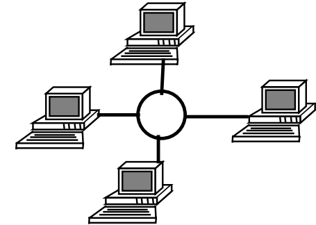
Token Ring
